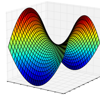
Surface z = x^2 - y^2
