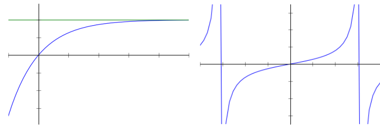
FIGURE 3 – Asymptotes
